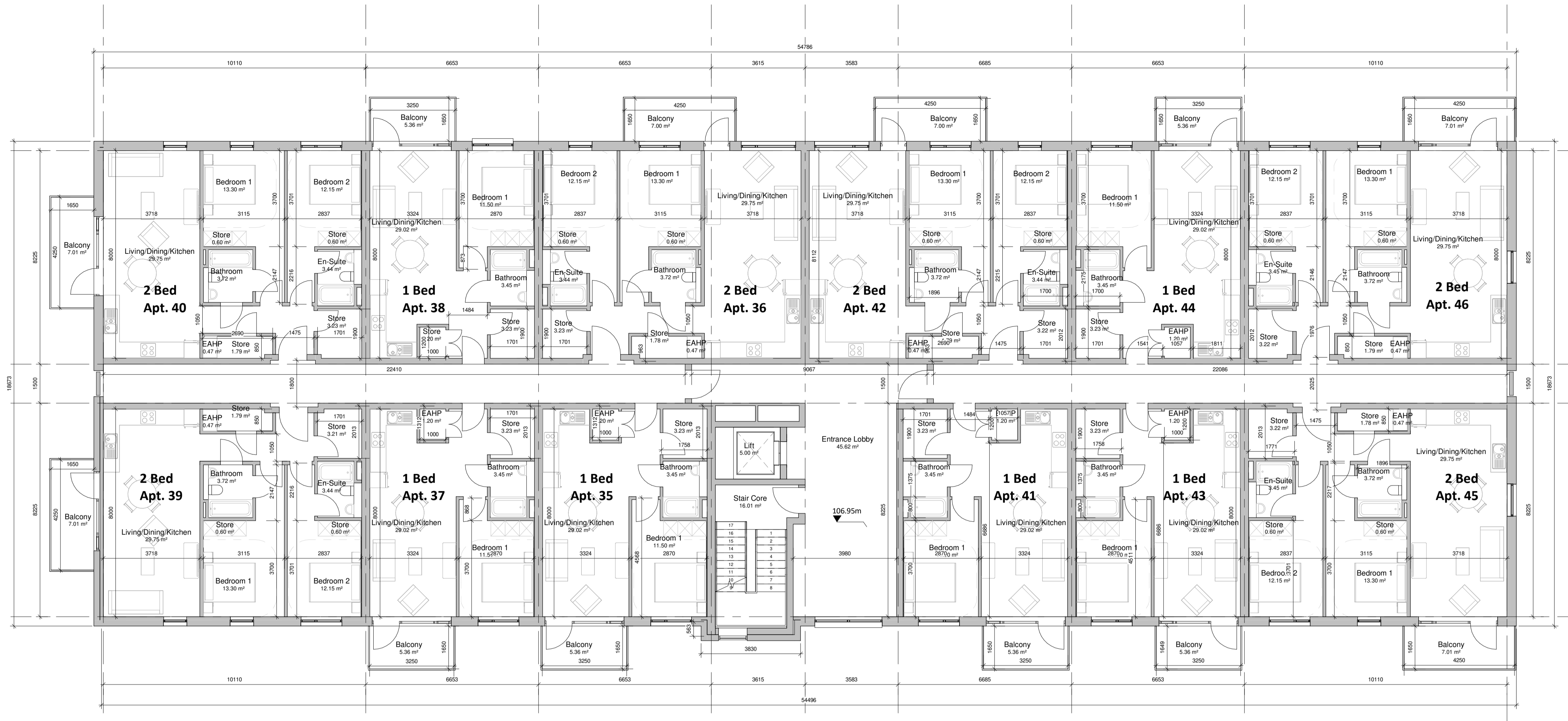
1 THIRD FLOOR LEVEL - BLOCK A 1 : 100
